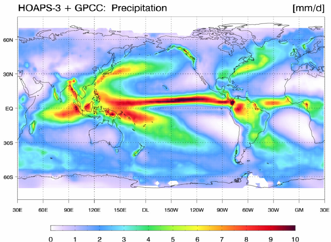
Figure 1.2a: Annual average precipitation amount derived by blending GPCC with HOAPS-3. DWD will generate a blend of HOAPS-4 and GPCC, which will comprise 20y of global precipitation over land (GPCC) and ocean (HOAPS).
