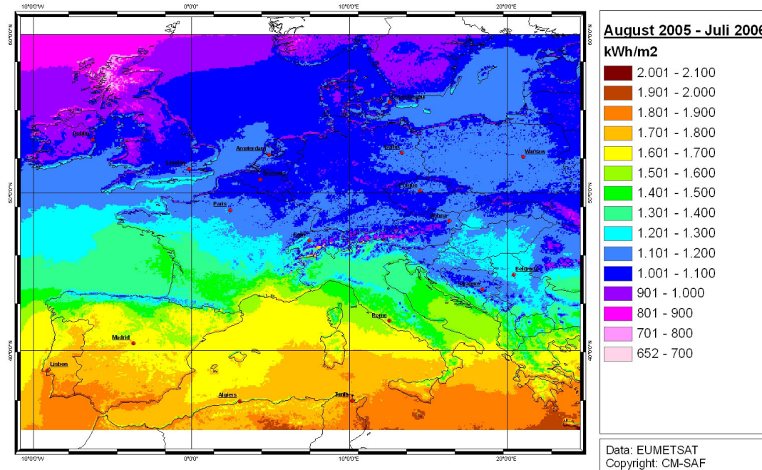
Figure 3.1a. Map of calculated solar energy in a typical year. Source: CM-SAF lead by DWD.
