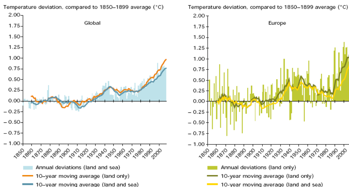
Figure 1.1a. Observed global and European annual average temperature deviations, 1850–2007 (EEA–JRC–WHO, 2008; Figure 5.2). The figure indicates that Europe warms more rapidly than the globe (+0.74°C over the last 100 years). The annual deviations are relative to the period 1850–1899 to better monitor the EU objective not to exceed 2 °C above pre-industrial values. Over Europe average annual temperatures during the real pre-industrial period (1750–1799) were very similar to those during 1850–1899. Source: UEA/Climate Research Unit ( www.cru.uea.ac.uk/cru/data/temperature/ ).
