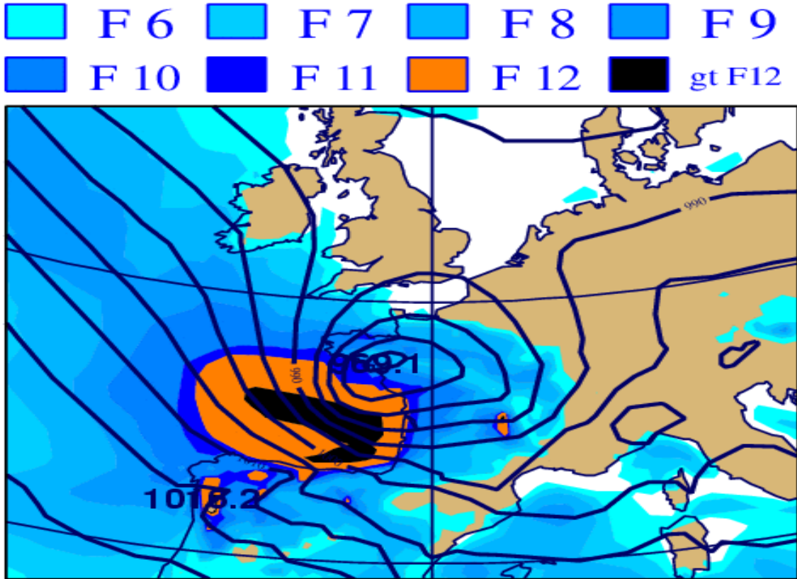
Figure 1.2c: Reconstruction of the 1999 “Christmas” storms using ERA-40 reanalysis data. This example shows the wind field of 27 December 1999 at 00 UTC. Colours indicate wind speed in Beaufort scale F (source: ECMWF).
