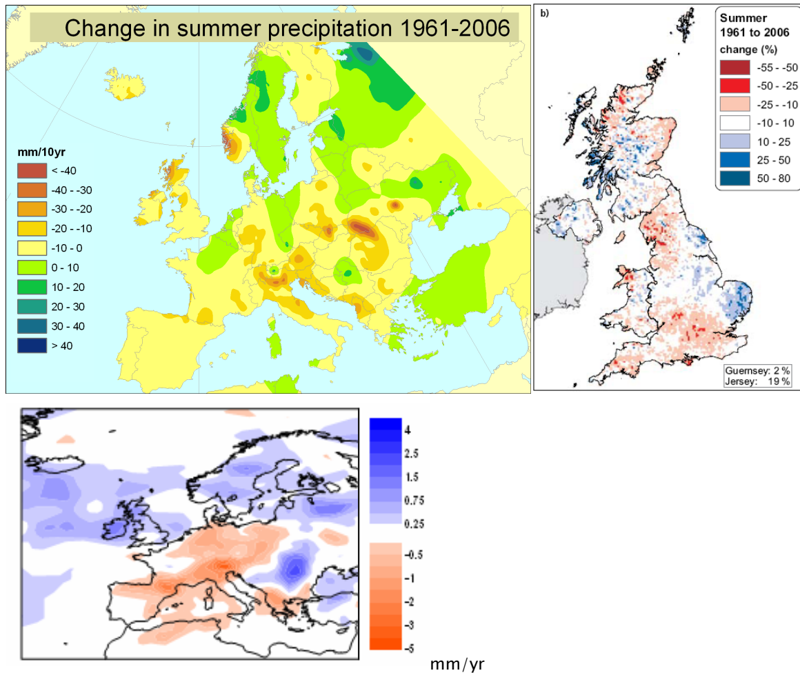
Figure 1.1c. Changes in summer (JJA) rainfall since 1961 estimated from different sources: a) the E-Obs dataset based on station observations (see Figure 1.1b); b) UKCIP08 (Jenkins et al. , 2007); c) ERA-40 reanalysis (ECMWF) The difference in trends over the UK illustrates the biases in existing global reanalysis products.
