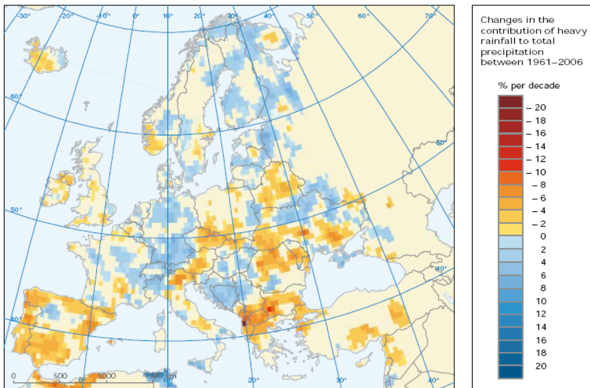
Figure 1.1b. Changes in the contribution of heavy rainfall to total precipitation 1961–2006 (EEA-JRC-WHO, 2008; Map 5.9). The figure indicates that the proportion of rainfall from heavy falls increases over most areas. Source: The E-Obs dataset from the EU-FP6 project ENSEMBLES ( www.ensembles-eu.org ) and the data providers in the ECA&D project ( eca.knmi.nl ).
