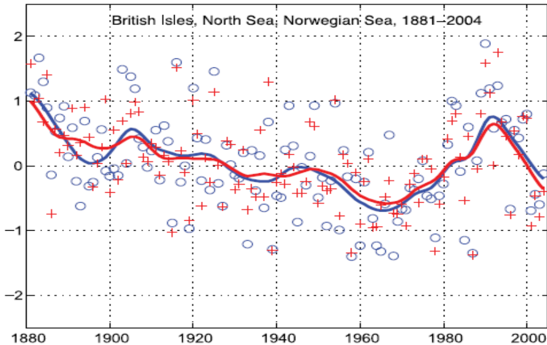
Figure 1.2b: Storm index for the British Isles, North Sea and Norwegian Sea, 1881 to 2004. Blue circles are 95th percentiles and red crosses 99th percentiles of standardised geostrophic winds averaged over 10 sets of triangles of stations. The smoothed curves are a decadal filter (updated by SMHI from Alexandersson et al. , 2000; see Figure 3.41 in IPCC-WGI-AR4).
